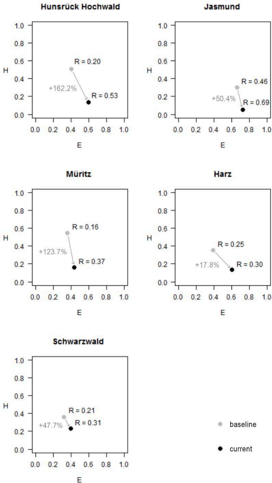
Figure 5: Panel showing the Rewilding Scores ( R ) for each time period (baseline, current) and their rewilding progress (%) over time in the bi-dimensional space created by the two main components of R , namely Human forcing ( H ) and Ecological Integrity ( E ), for each site.
